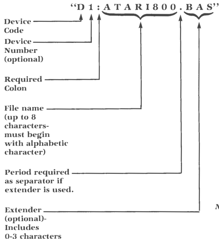
Figure 5-2 Filename Breakdown
