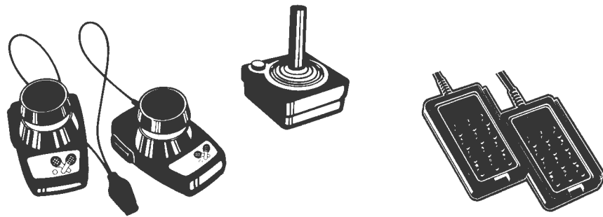
Figure 10-2. Game Controllers
