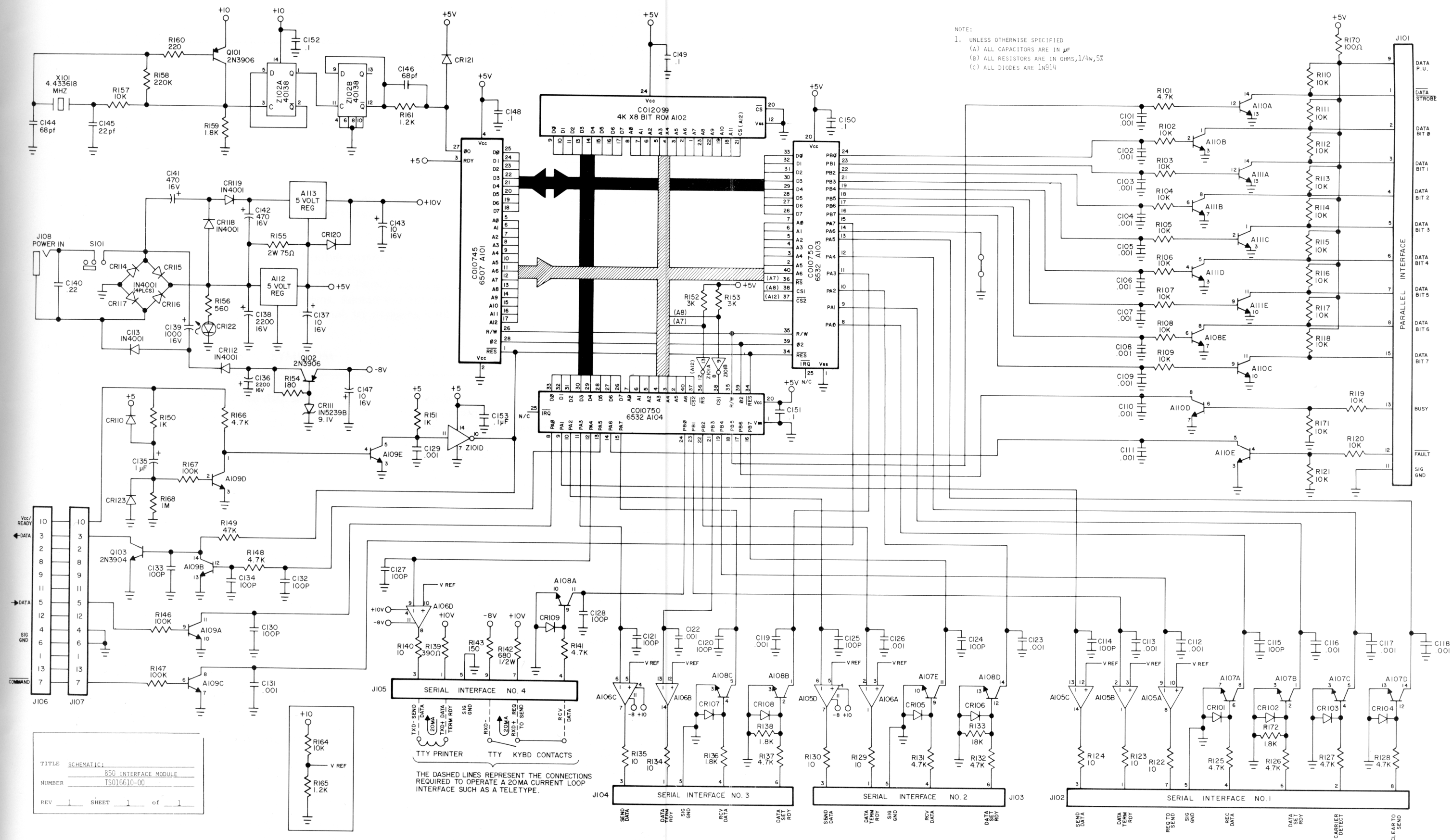
Figure C-6 Atari 850 Interface Module Schematic Diagram
